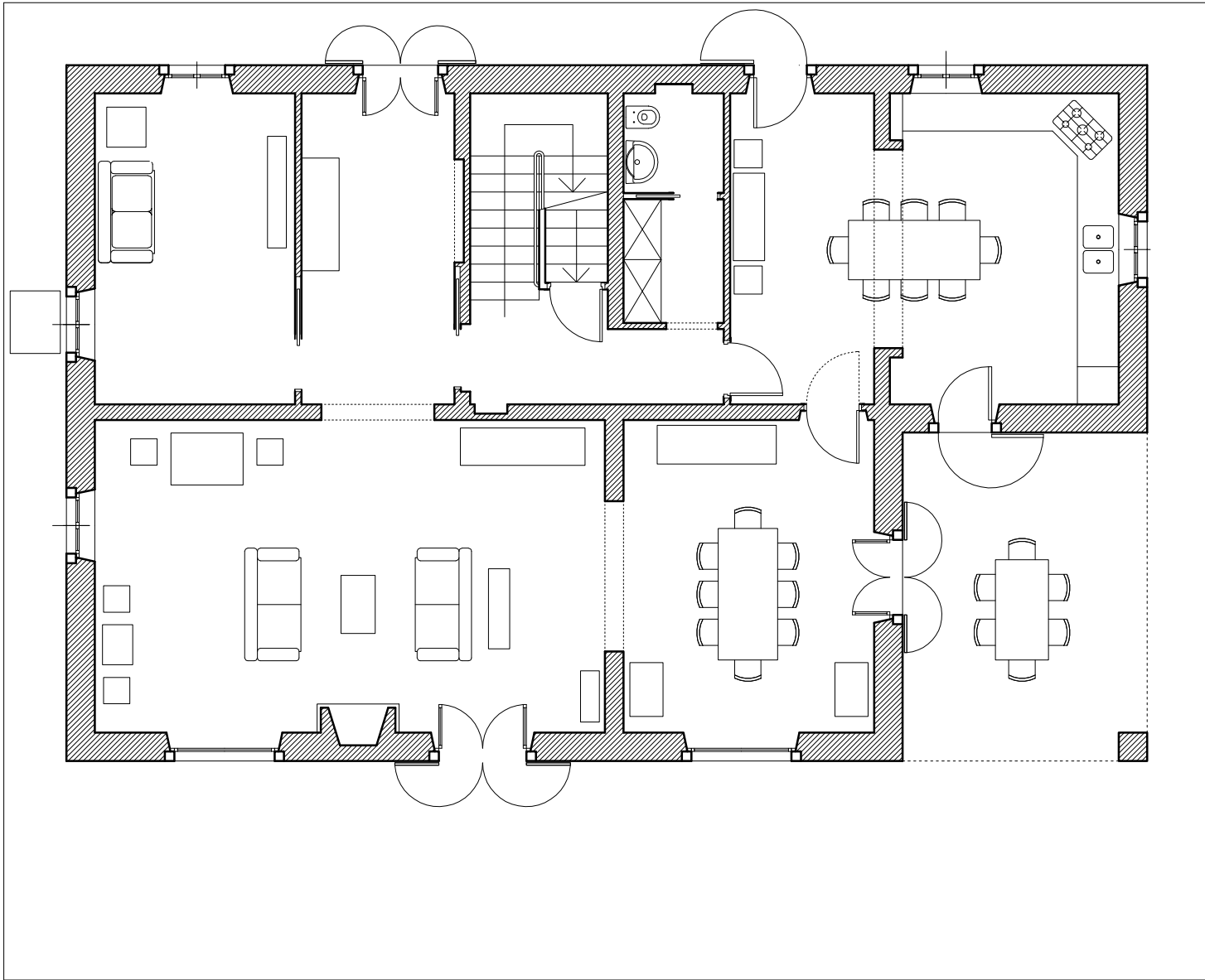
casa C ground floor
